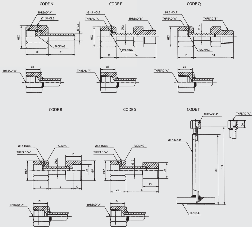
Dimensions (mm)
